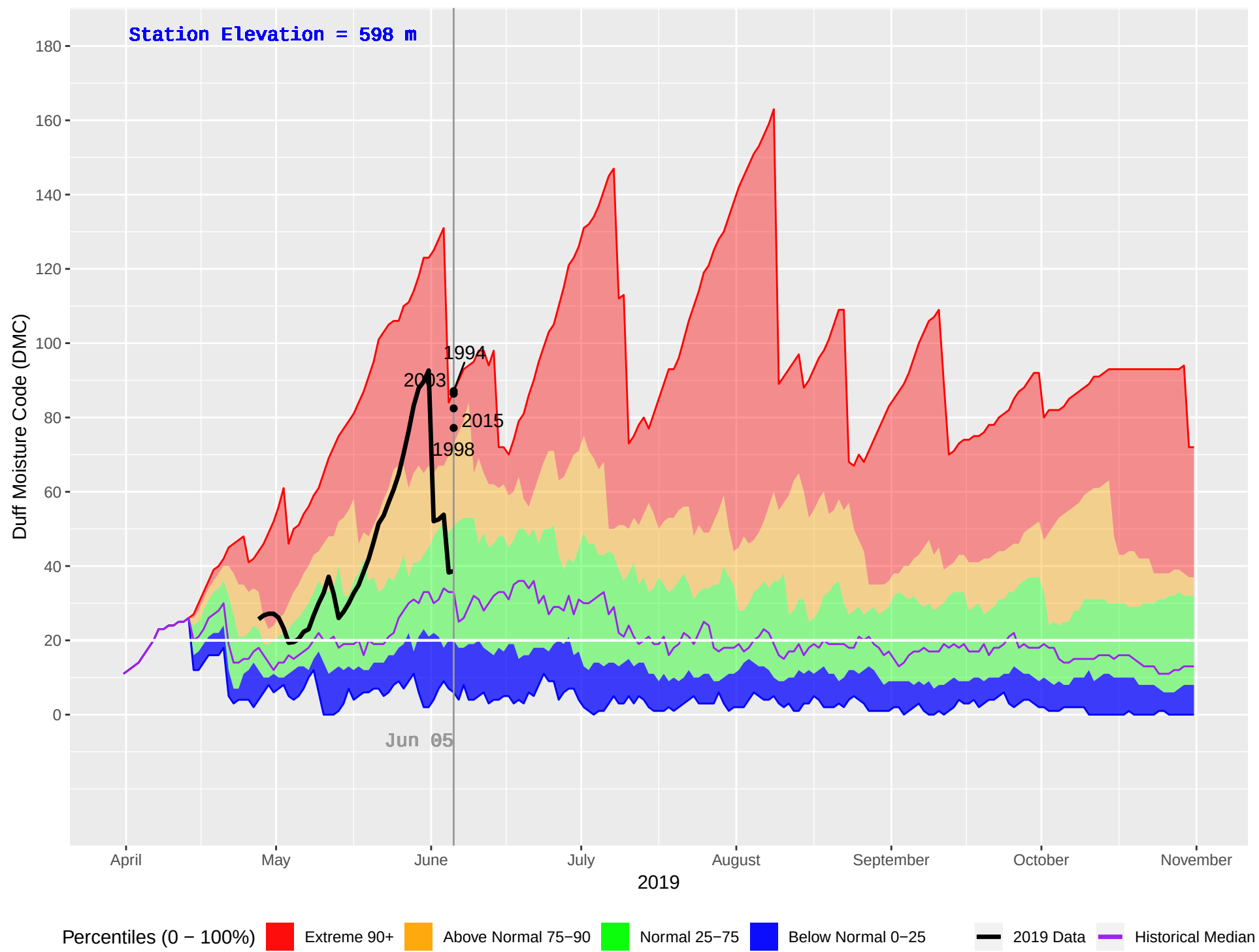
HELMUT (118) : Historical (1983–2018), Current (2019) Daily Duff Moisture Code (DMC)
