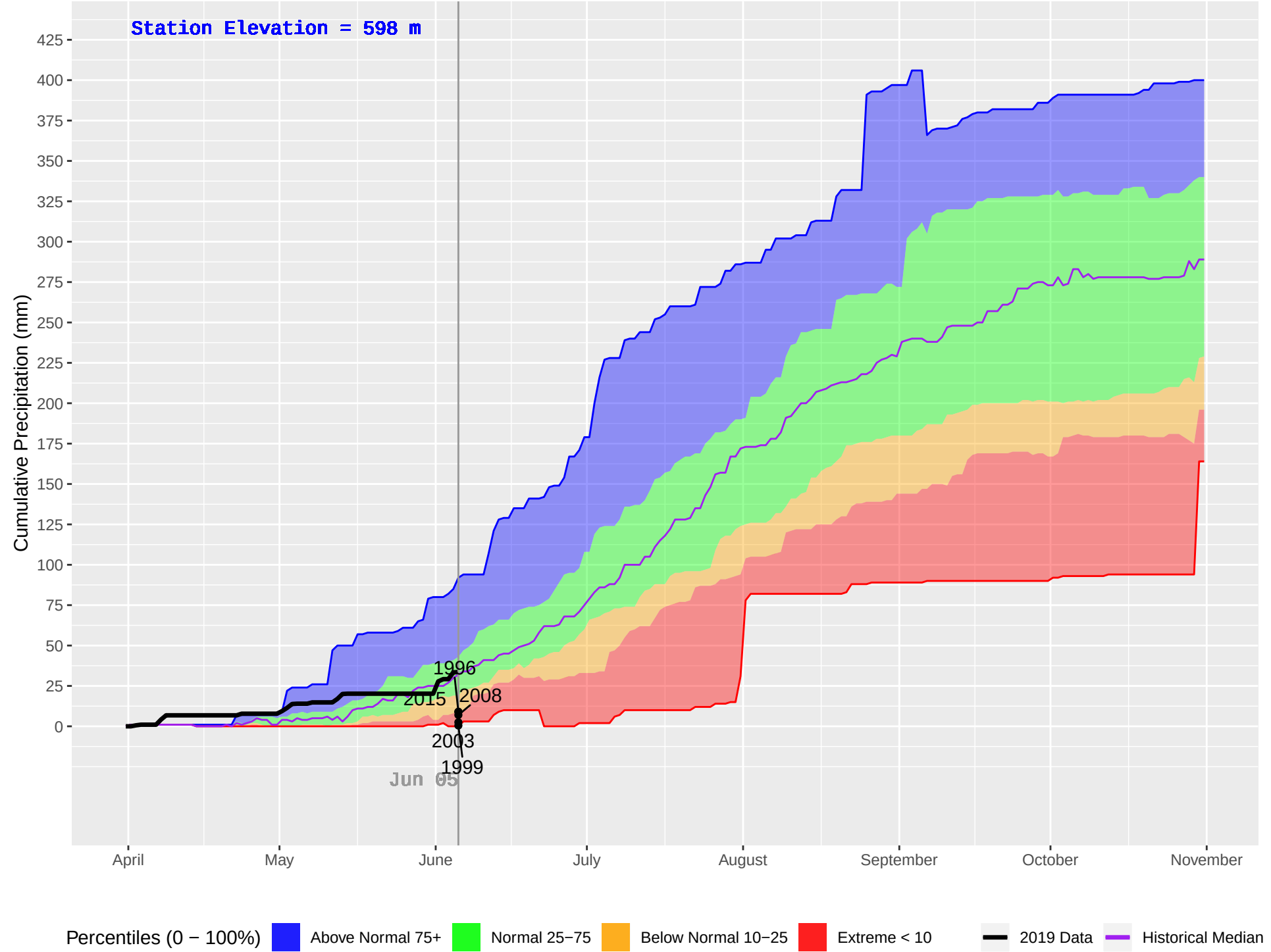
HELMUT (118) : Historical (1983–2018), Current (2019) Daily Cumulative Precipitation
