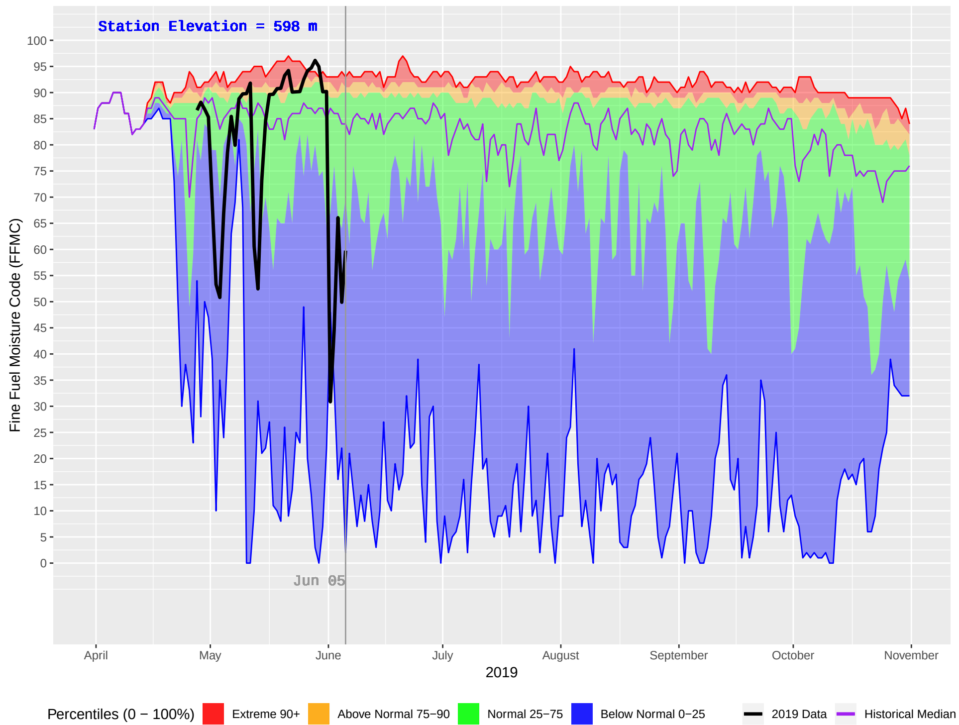
HELMUT (118) : Historical (1983–2018) and Current (2019) Daily Fine Fuel Moisture Code (FFMC)
