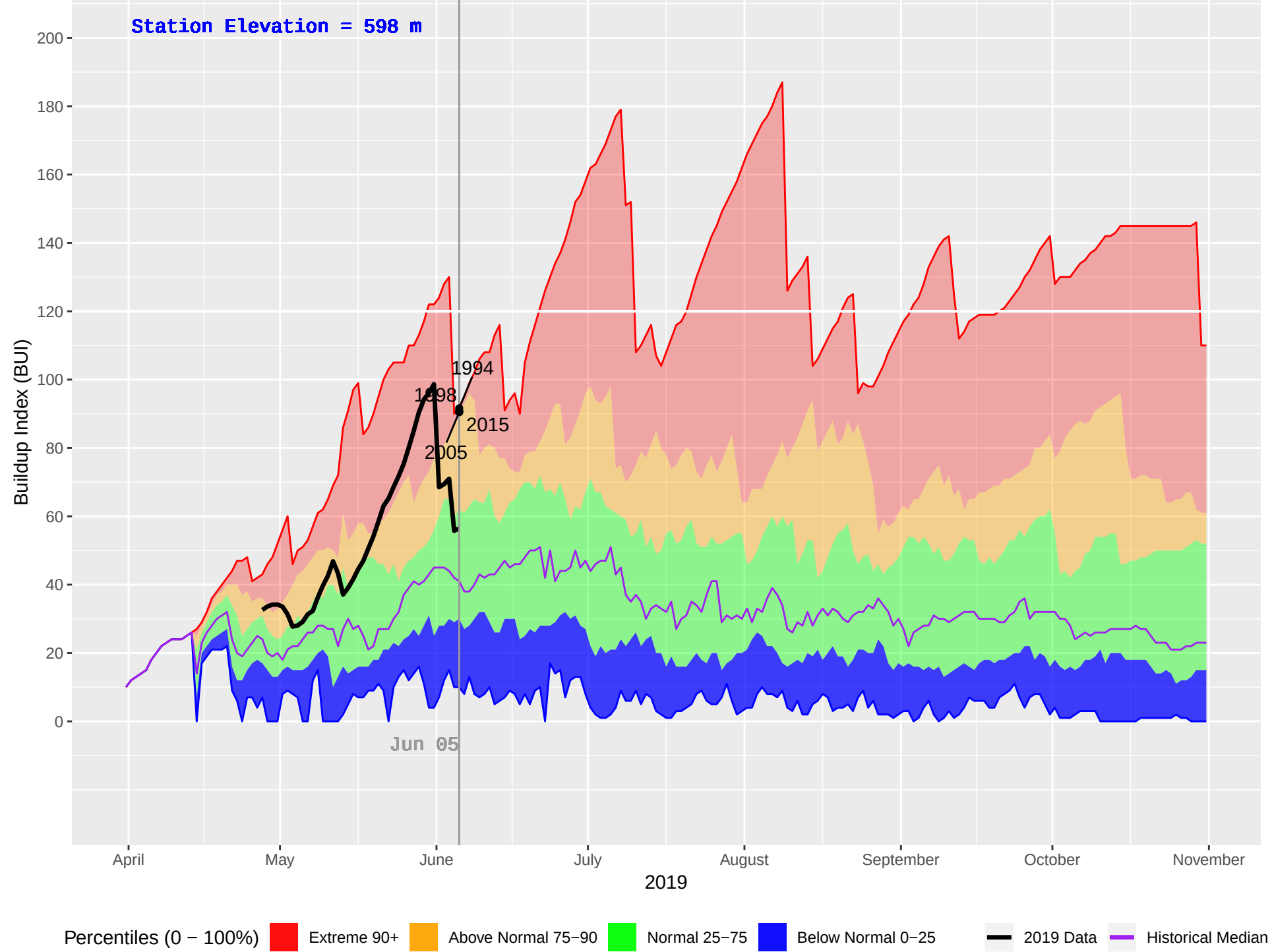
HELMUT (118) : Historical (1983–2018), Current (2019) Daily Buildup Index (BUI)
