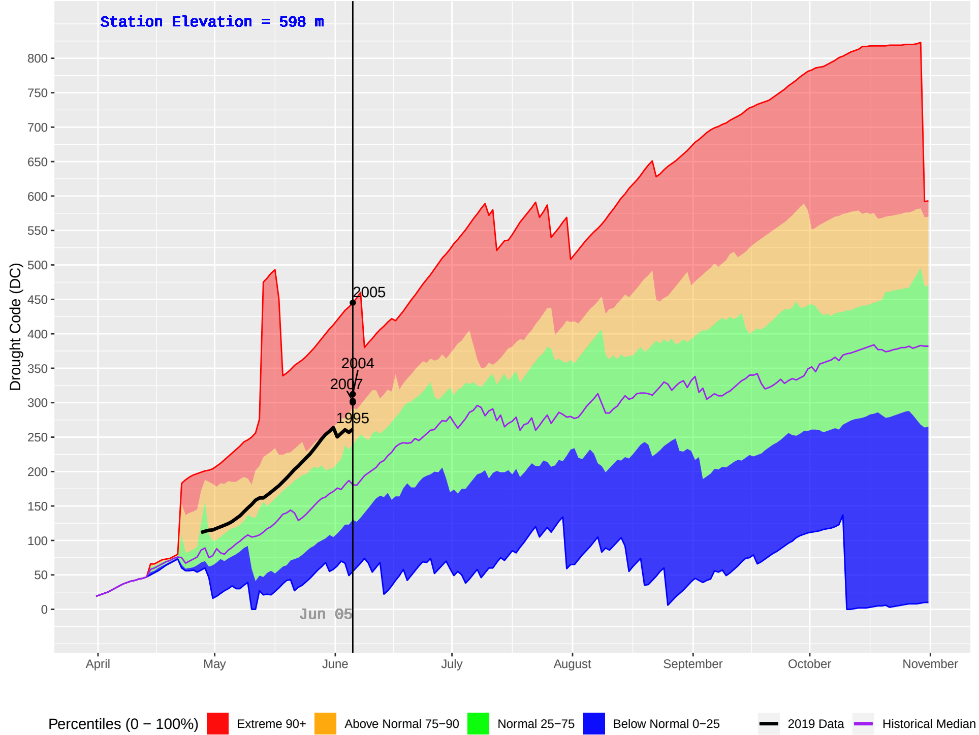
HELMUT (118) : Historical (1983–2018) and Current (2019) Daily Drought Code (DC)
